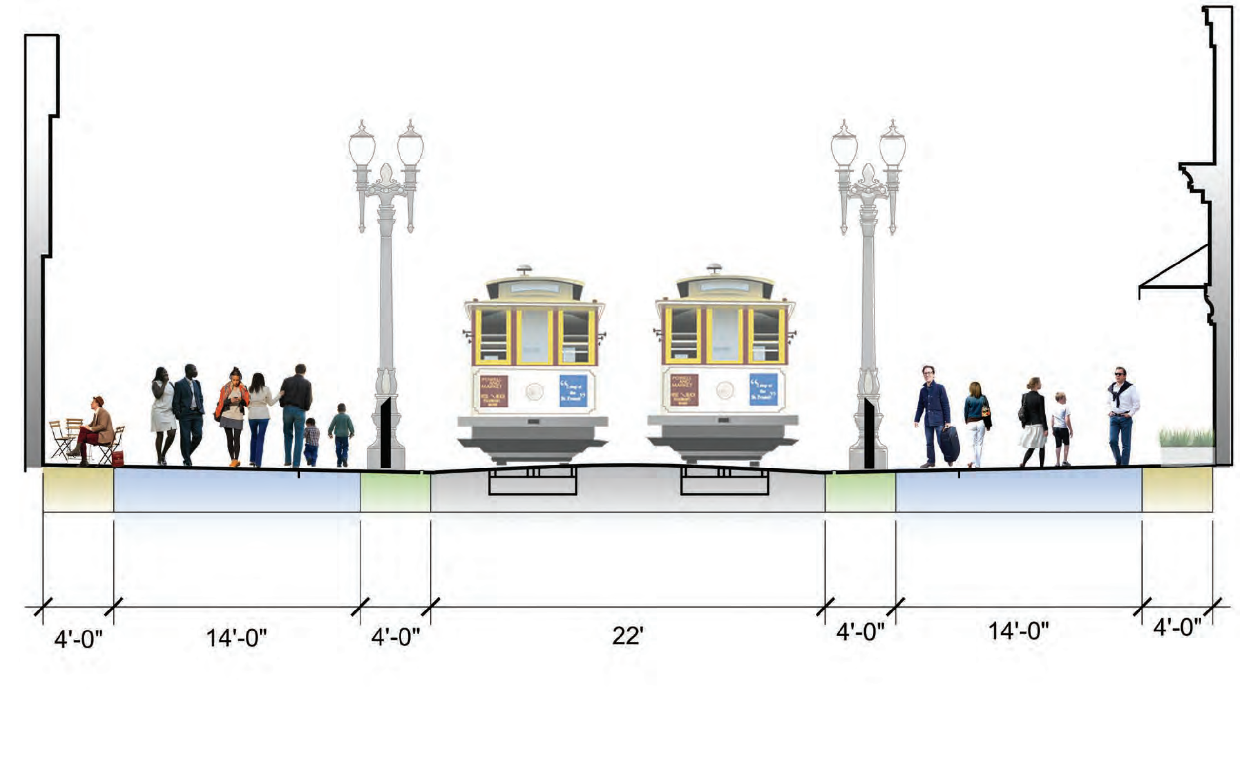
(A) TYPICAL SECTION
