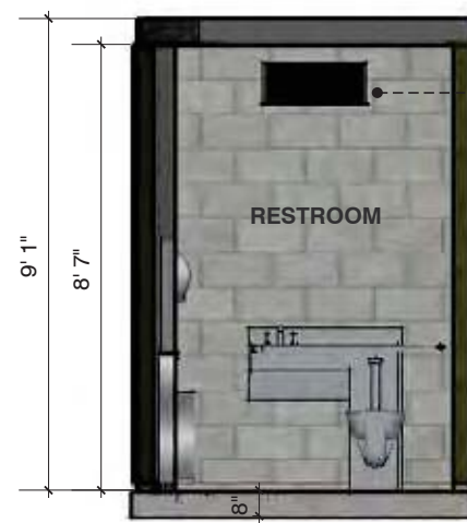
TRANSVERSE SECTION
