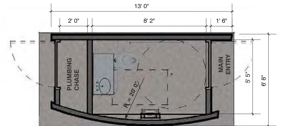
FLOOR PLAN - SINGLE OCCUPANCY- BASIC MODULE
