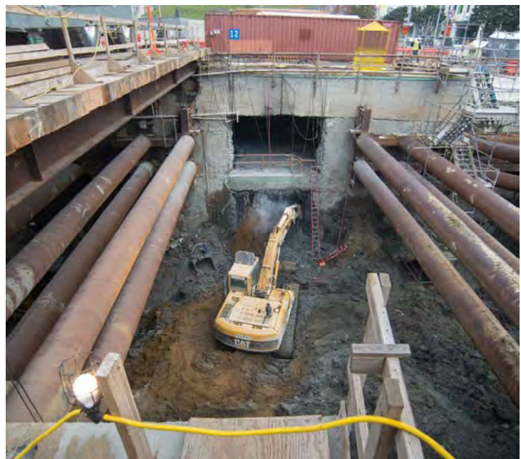
3 A new access portal is created in the slurry wall to excavate the next level.
