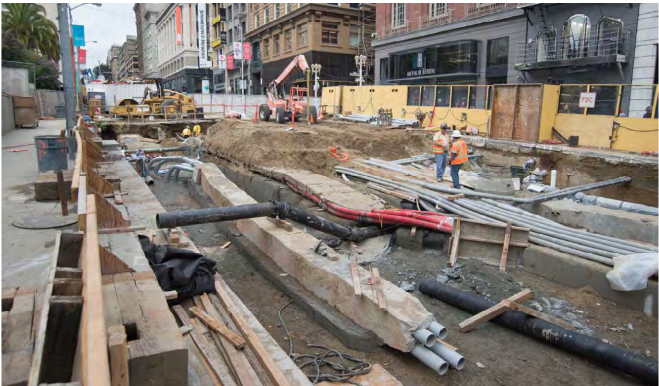
Exposed utilities formerly suspended from a steel truss lattice while excavation went on below now rest atop the roof deck of the north station concourse.
