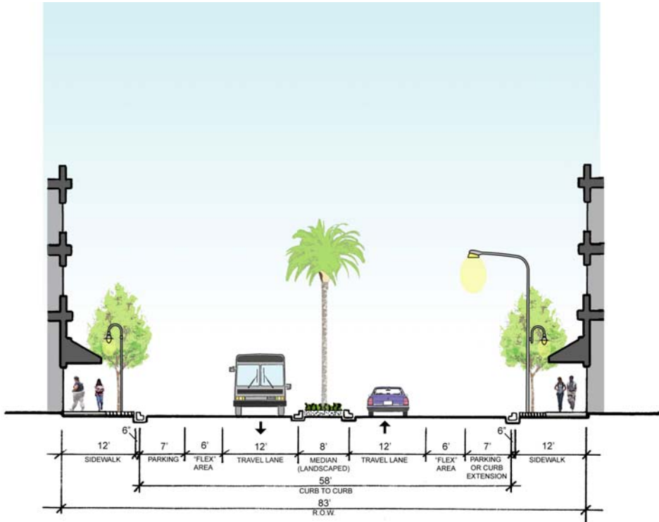
Figure 3.1 – Cross-section view of recommendation for Mission Street
