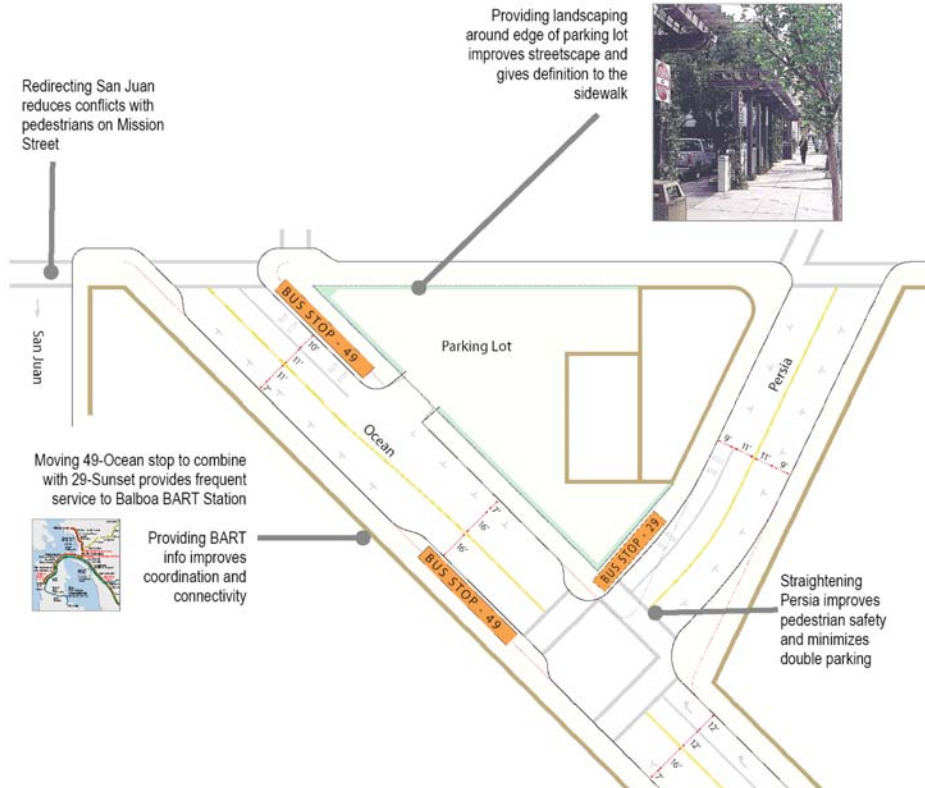
Figure 5.1 - Proposed Improvements to Persia Triangle
