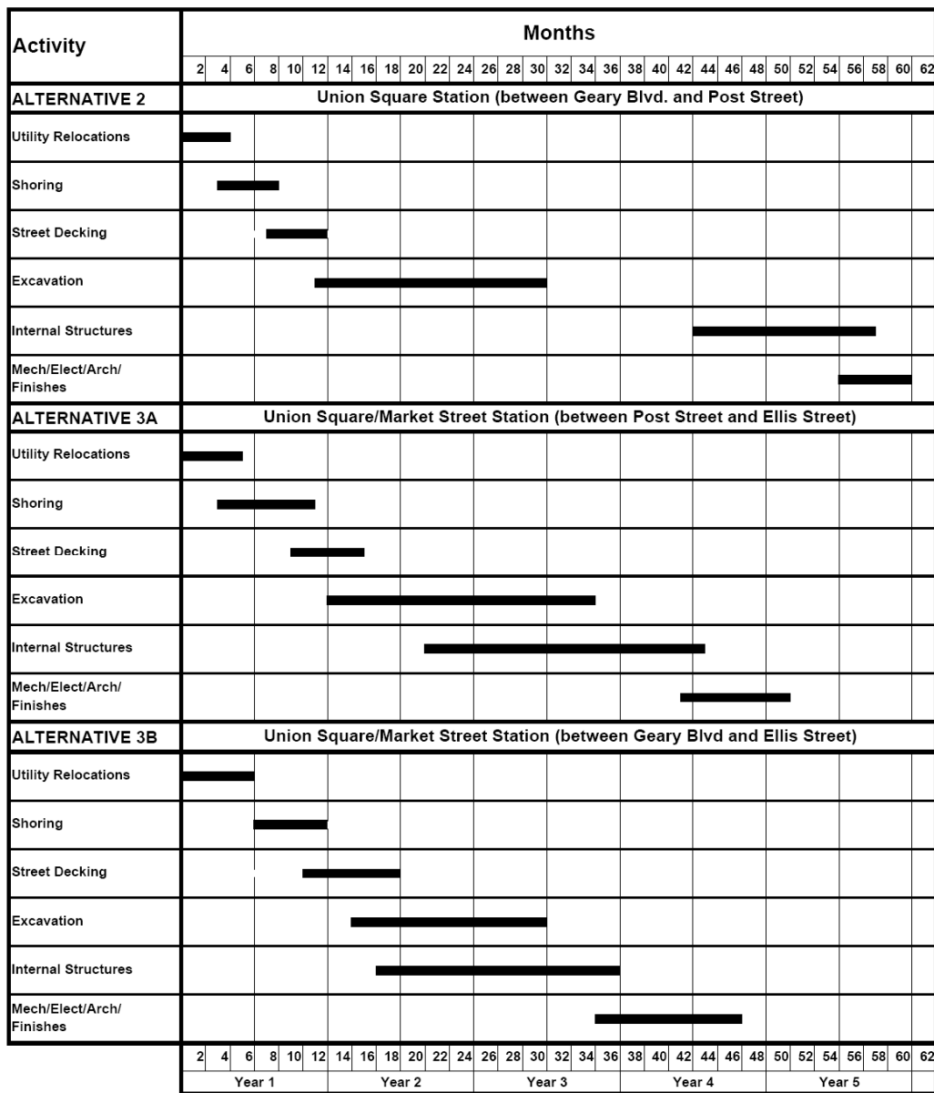
FIGURE 6-10 CONSTRUCTION ACTIVITIES AND DURATIONS FOR UNION SQUARE AND UNION SQUARE/MARKET STREET STATIONS
