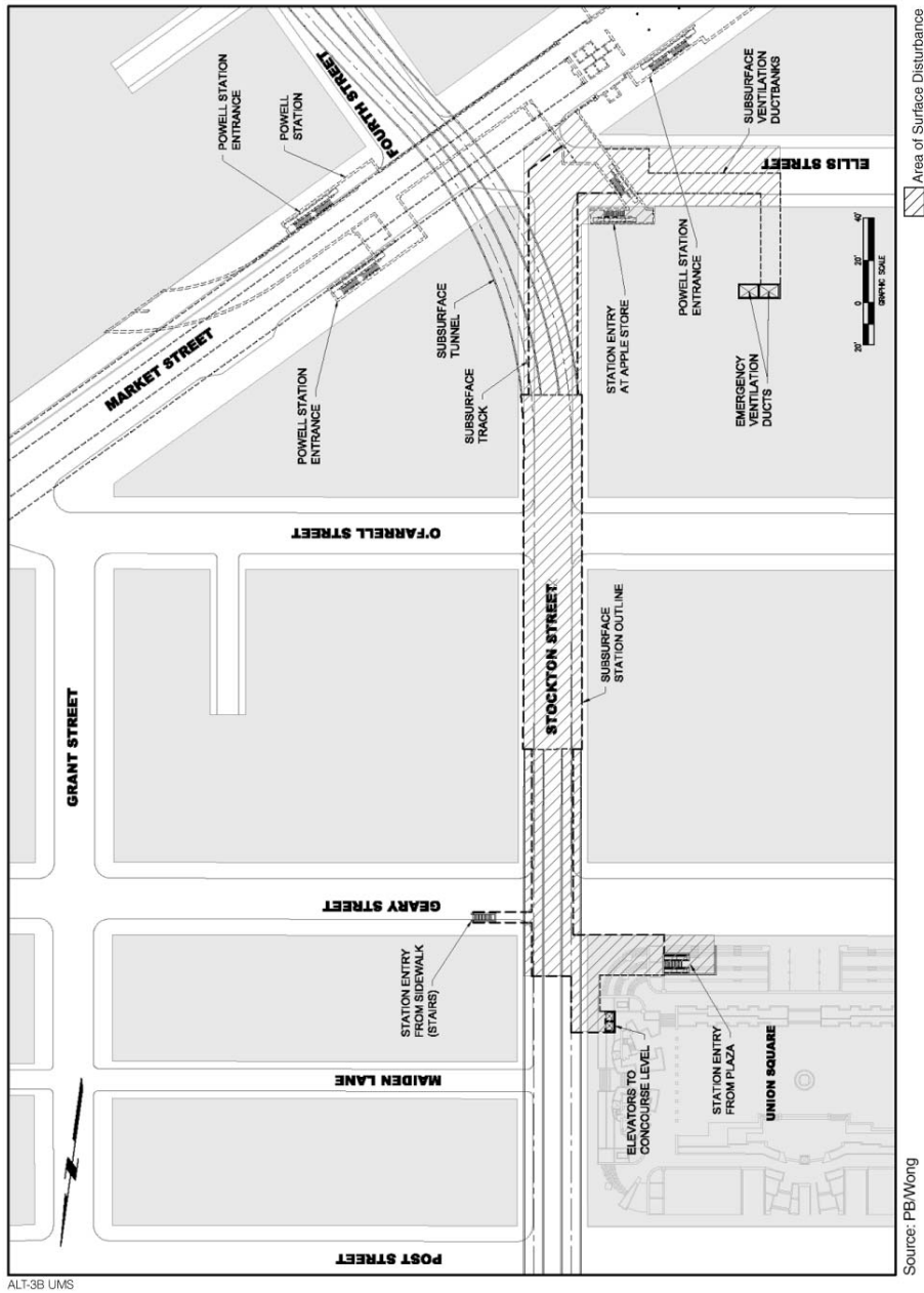
FIGURE 6-15 ALT. 3B UNION SQUARE/MARKET STREET STATION AREA OF SURFACE DISTURBANCE DURING CONSTRUCTION
