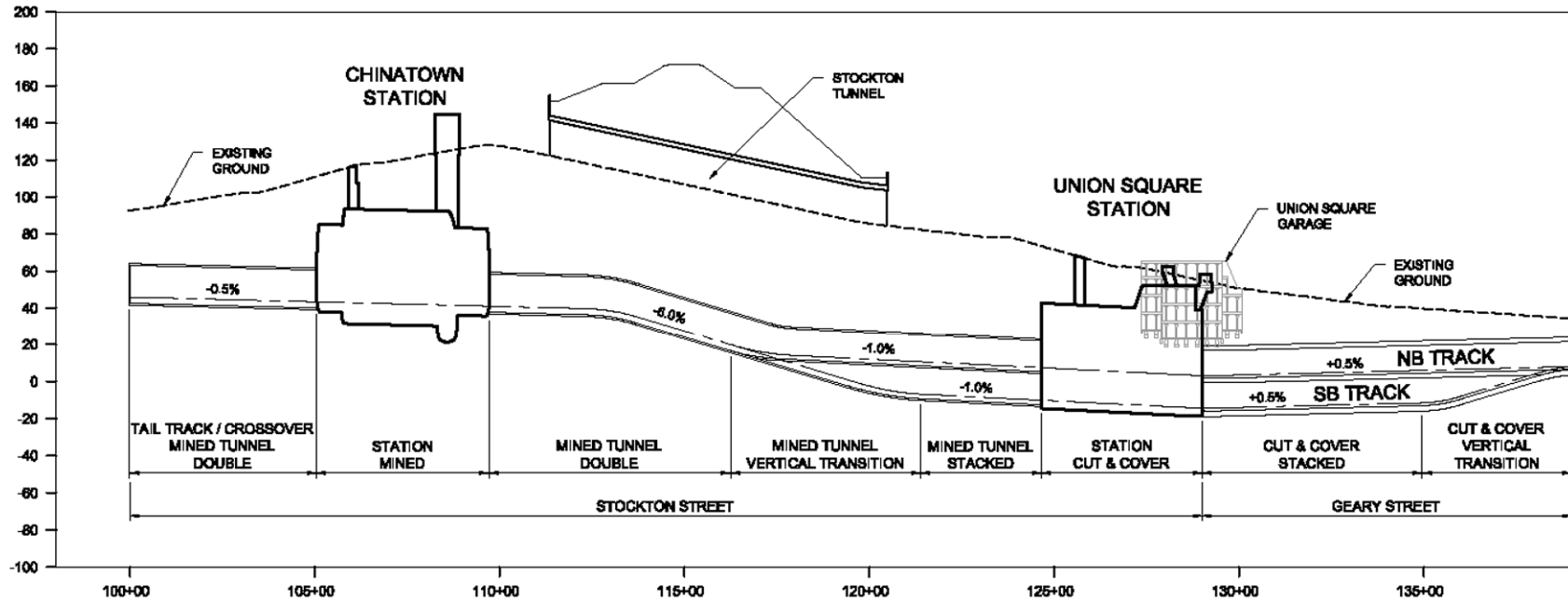
FIGURE 2-6: ENHANCED EIS/EIR ALIGNMENT PROFILE BETWEEN MARKET/THIRD STREET AND STOCKTON/JACKSON STREETS
