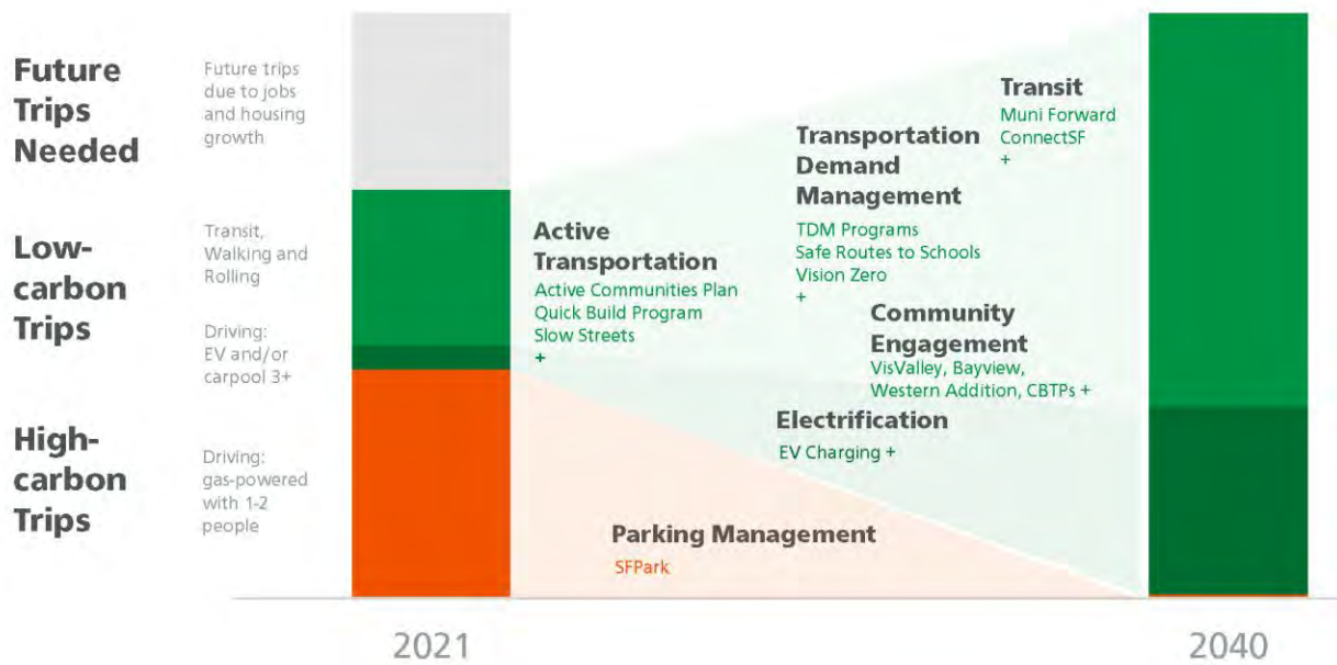
Scenario to Get to Net-zero Greenhouse Gas Emissions from Ground Transportation
