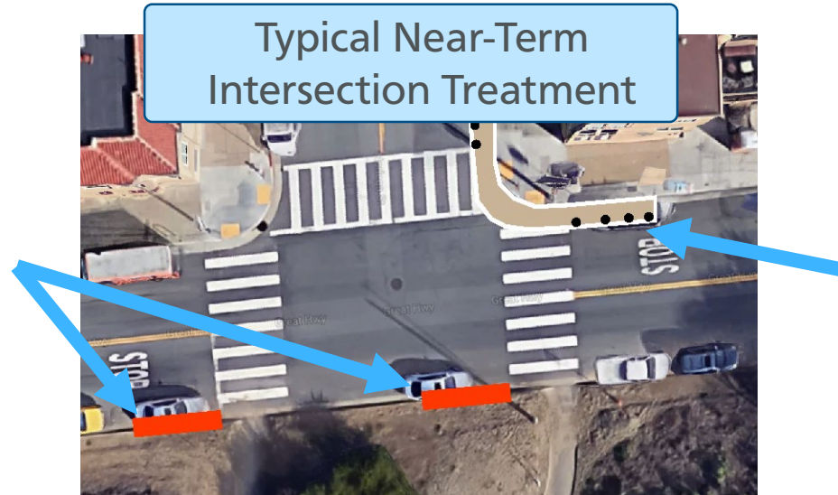
Pedestrian Visibility Zones (Daylighting)
