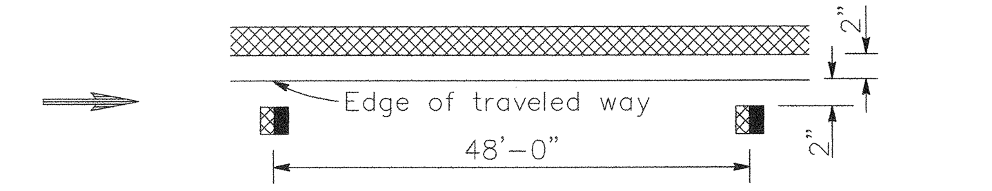
DETAIL 25: LEFT EDGE LINE (DIVIDED HIGHWAYS) (4" SY)
