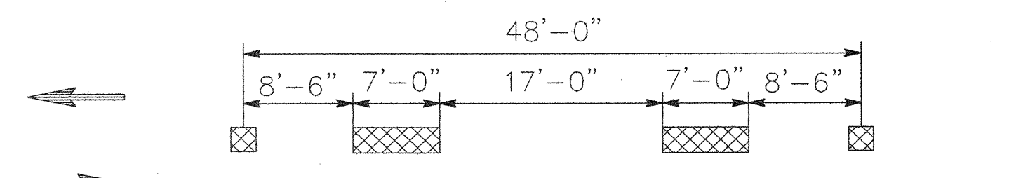
DETAIL 2: CENTERLINE ON TWO LANE CONVENTIONAL HIGHWAYS (4" BY)
