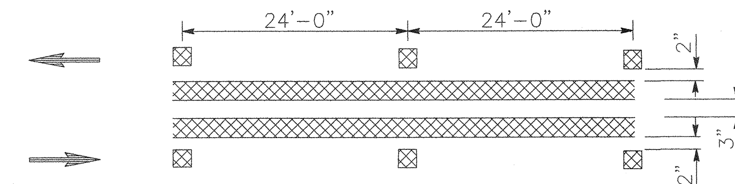
DETAIL 22: TWO-WAY NO PASSING ZONE WITH PAINTED STRIPE (DY)
