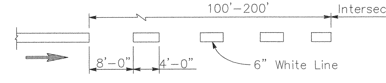
DETAIL 39A: BIKE LANE - INTERSECTION LINE (6" BW)
