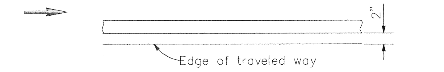
DETAIL 27B: RIGHT EDGE LINE (4" SW)
