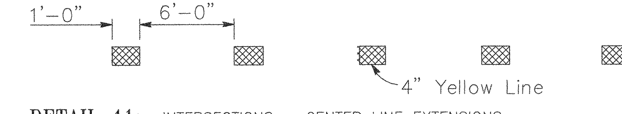
DETAIL 41: INTERSECTIONS - CENTER LINE EXTENSIONS
