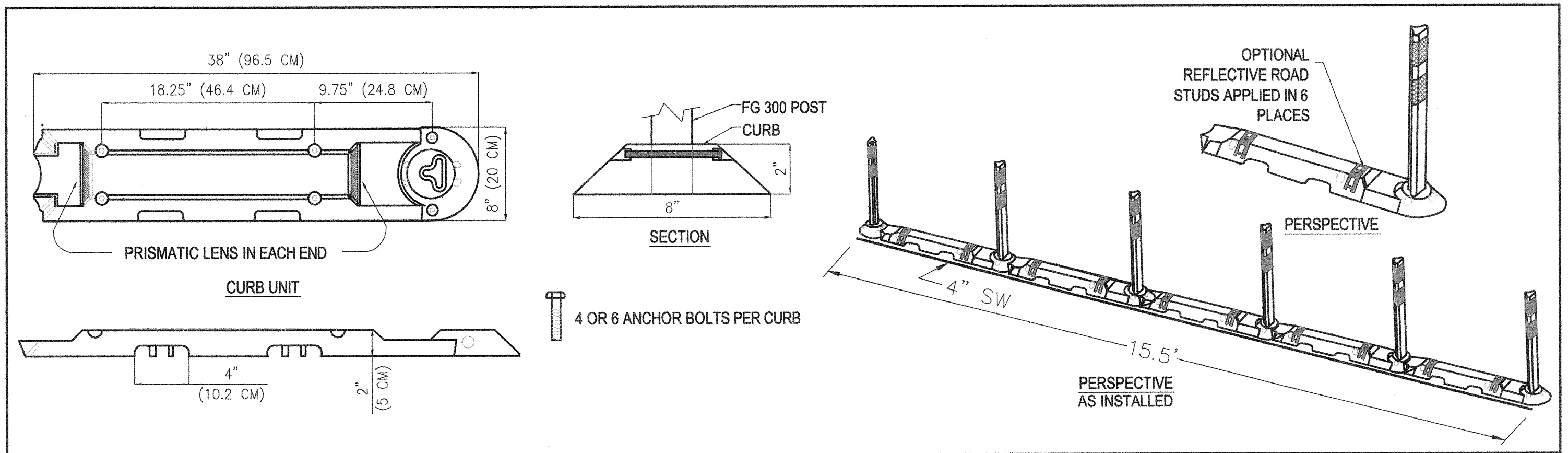
DETAIL A: 15.5' RAISED MOUNTABLE WHITE CURB DETAILS (NTS)
