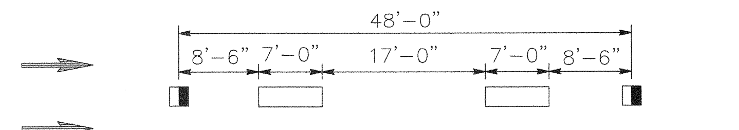
DETAIL 9: LANE LINE ON MULTILANE HIGHWAYS (4" BW)
