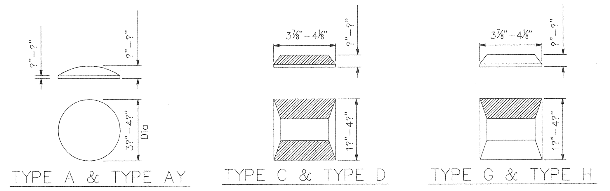
TYPE A & TYPE AY TYPE C & TYPE D TYPE G & TYPE H Retroreflective Face MARKER DETAILS
