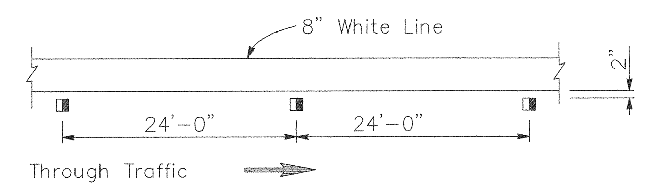
DETAIL 38: 8" WHITE CHANNELIZATION STRIPE (8" SW FOR TURN POCKETS)
