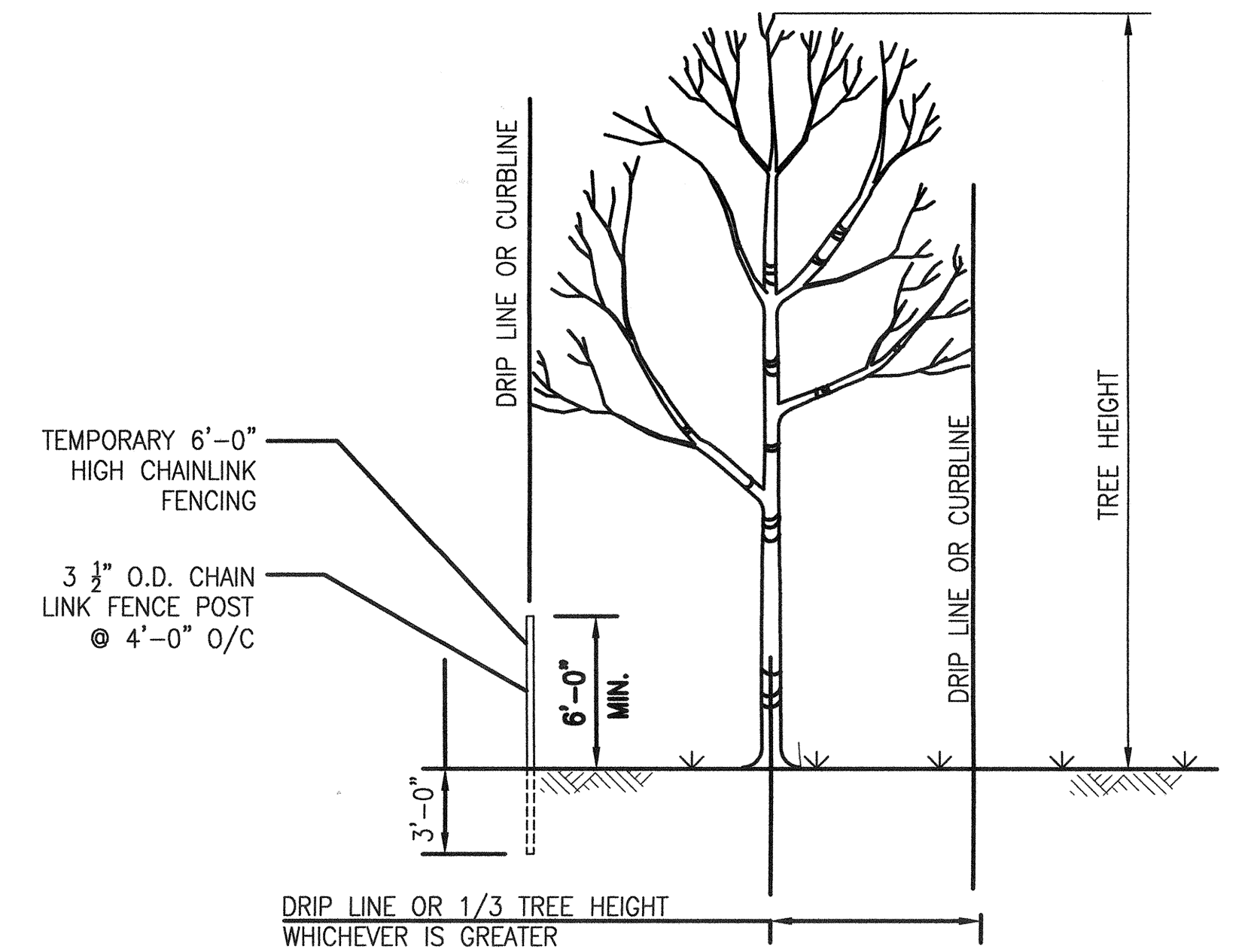
TYPICAL EXISTING TREE PROTECTION NO SCALE NOTE: SIDEWALK TREES TO RECEIVE TREE PROTECTION FENCING AS DIRECTED BY CITY REPRESENTATIVE
