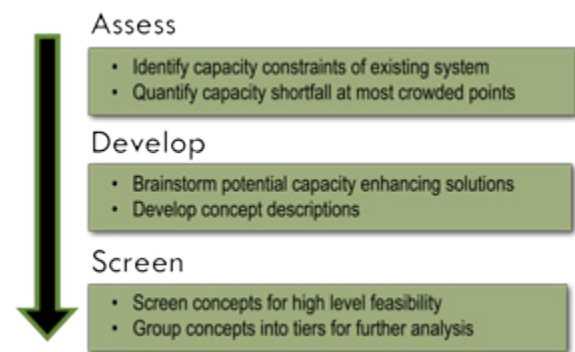
Figure 2.1 Methodological Process
