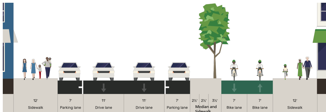
Karaniwang Cross-section ng Howard Streetscape Project
