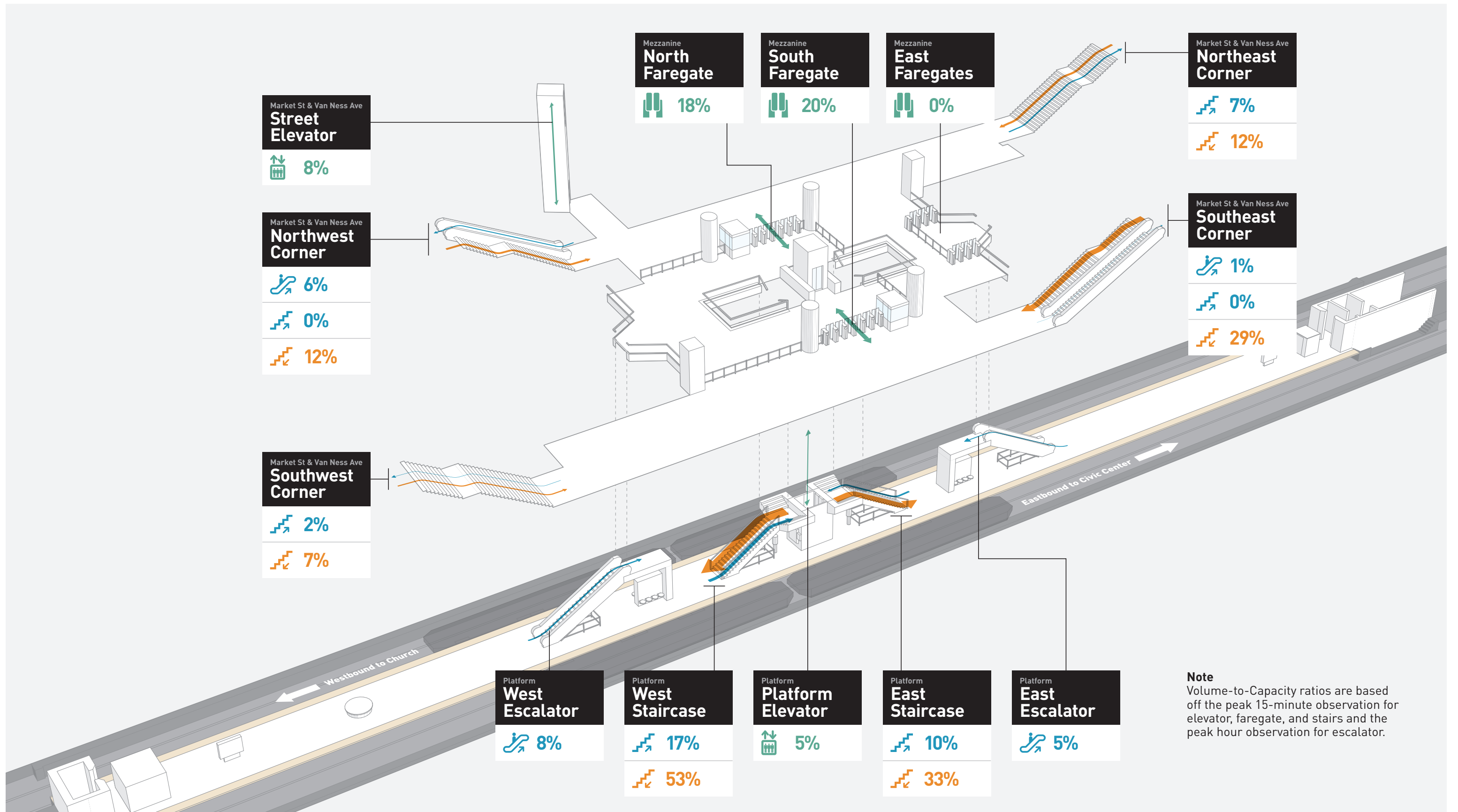
Figure 2 Van Ness Station PM Peak Period Volume-to-Capacity Ratio for Key Station Elements
