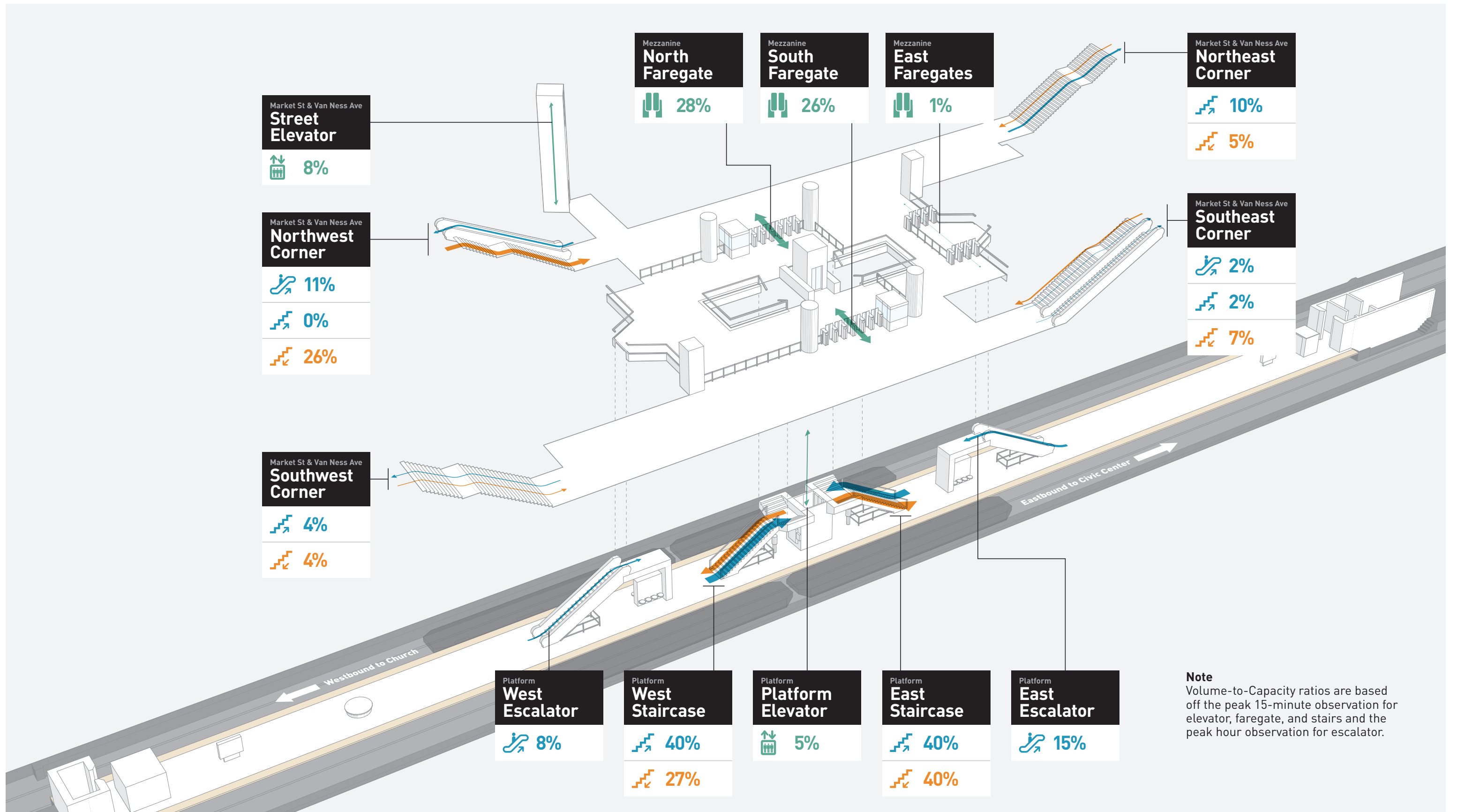
Figure 1 Van Ness Station AM Peak Period Volume-to-Capacity Ratio for Key Station Elements
