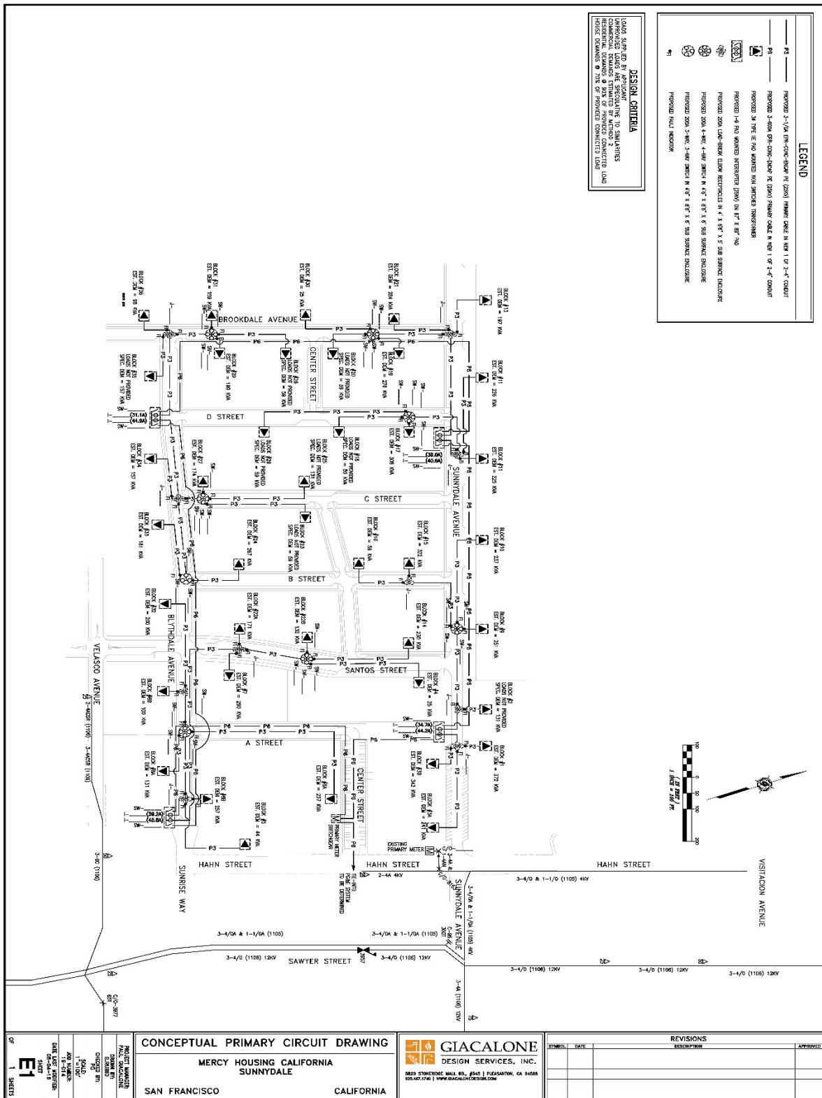
Figure 14.4 Conceptual Joint Trench Plan
