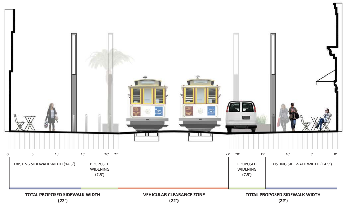
SECTION B
