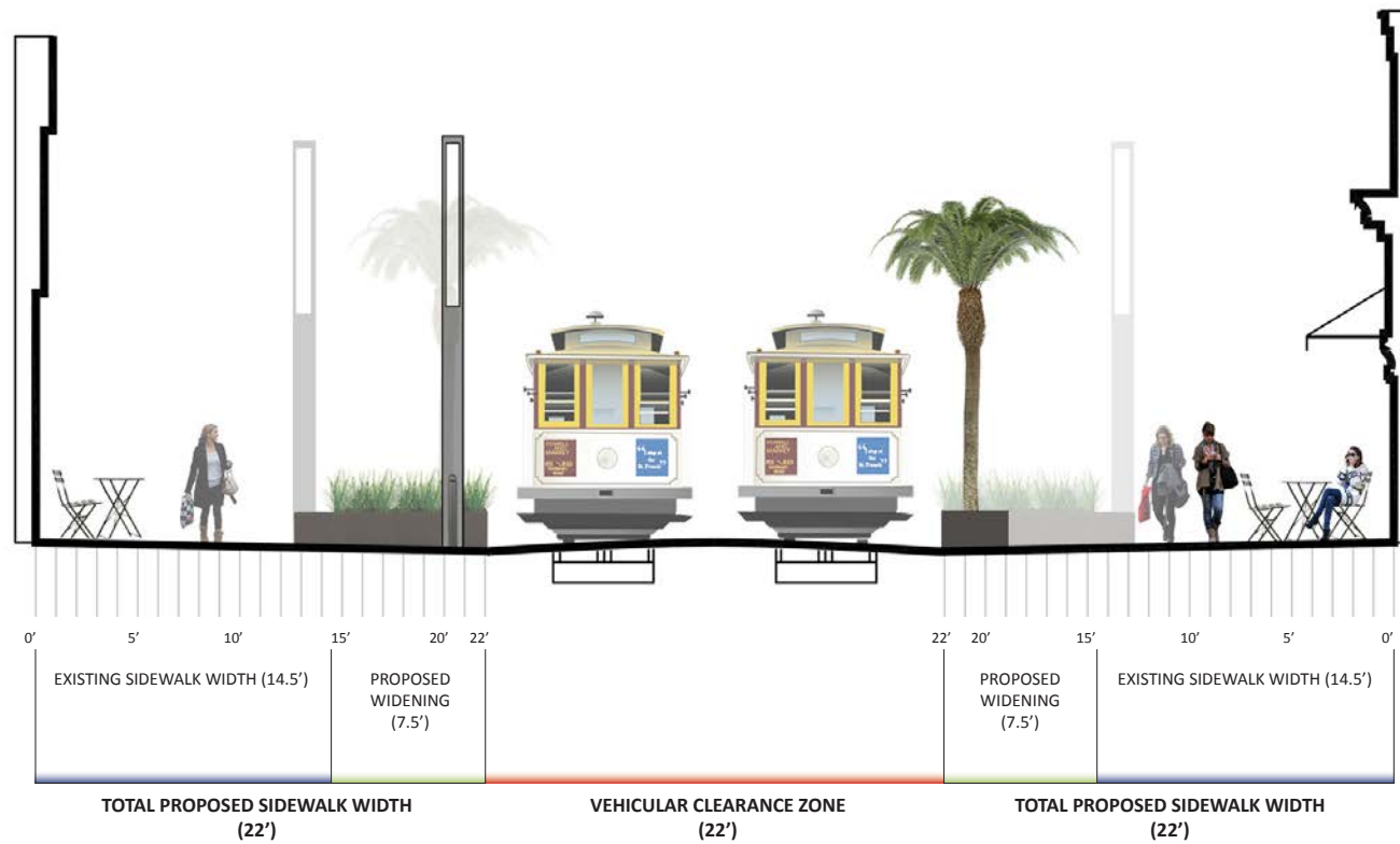
SECTION A
