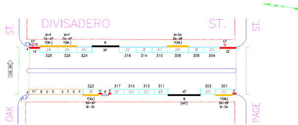
METER DRAWING - EXISTING CONDITIONS
