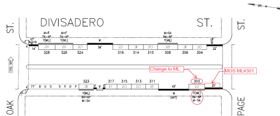
METER DRAWING - PROPOSED CONDITIONS
