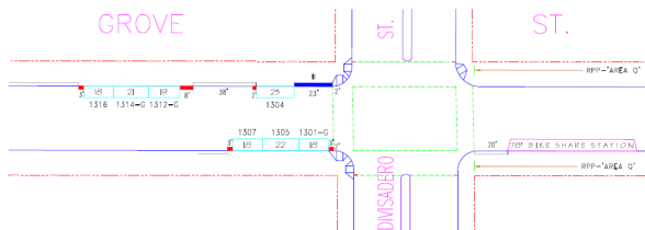
METER DRAWING - PROPOSED CONDITIONS
