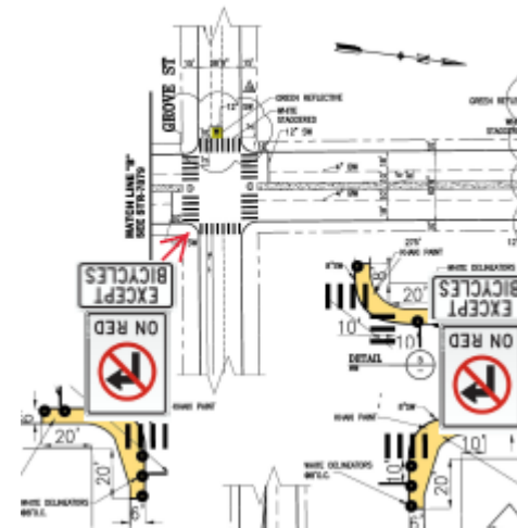
PROPOSED DESIGN - BIKE BOXES
