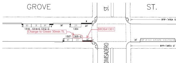
METER DRAWING - PROPOSED CONDITIONS
