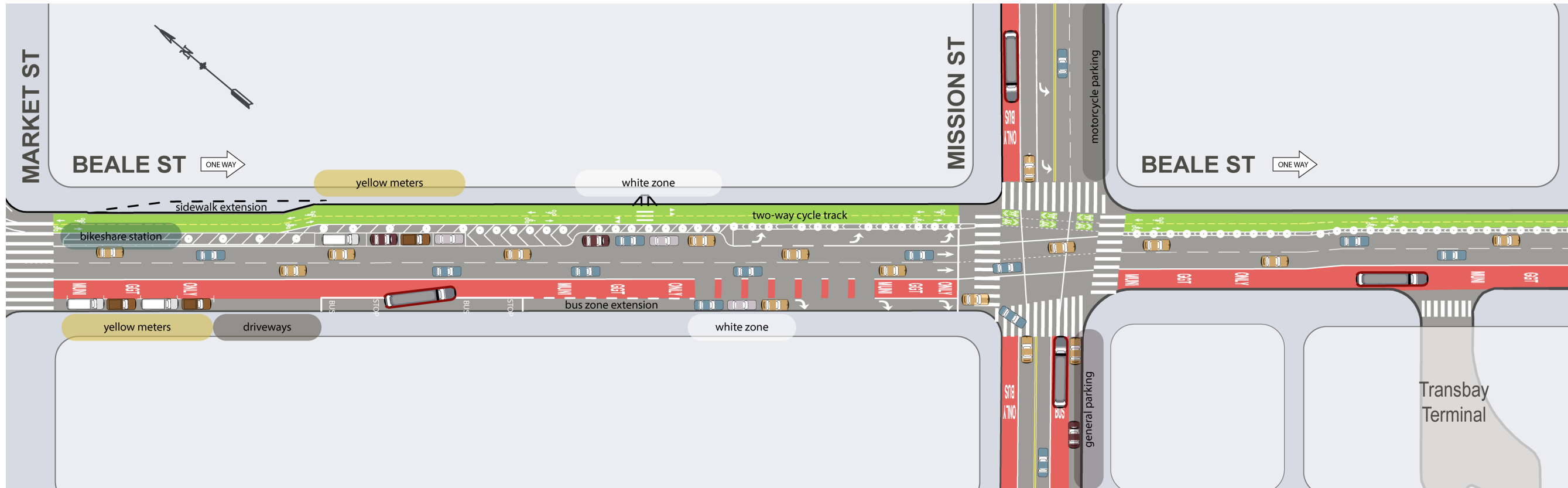
Above: Beale Street with proposed transit-only lane, two-way cycle track between Market and Natoma streets.
