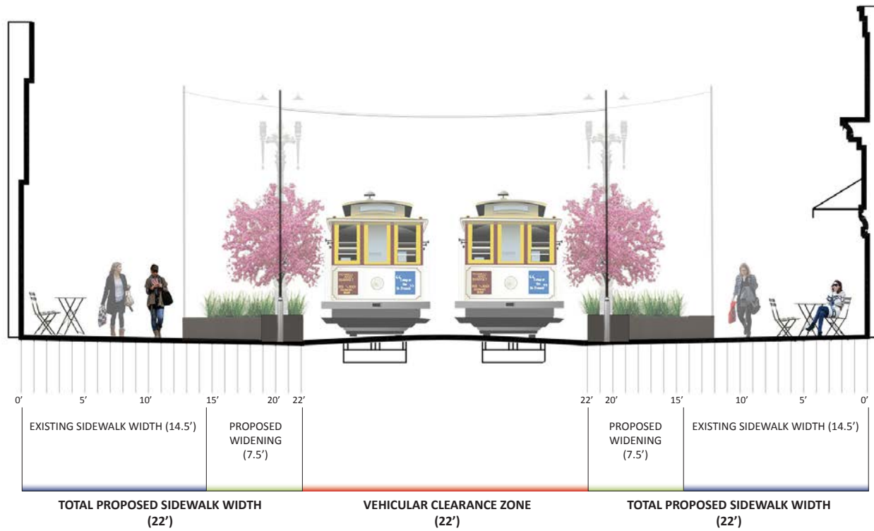
SECTION A
