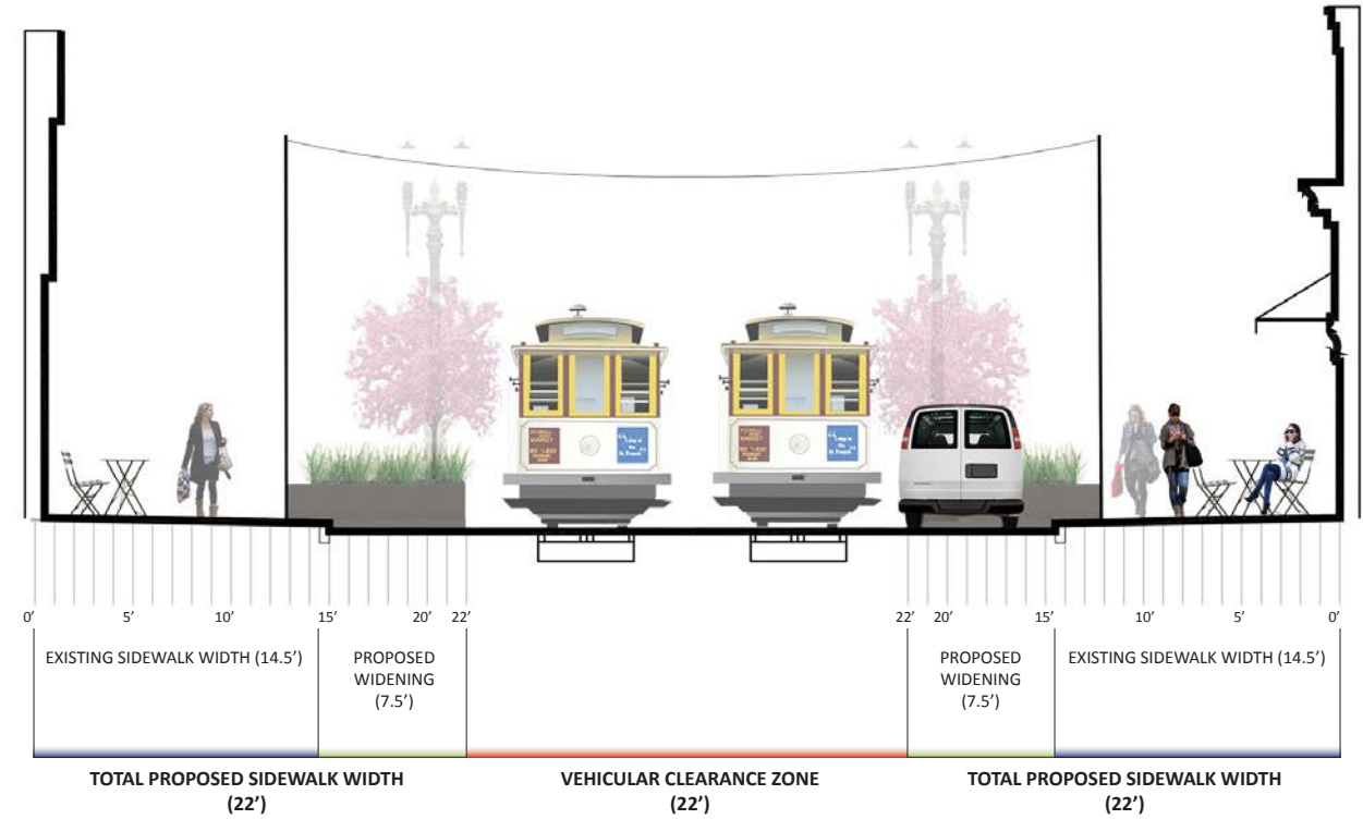
SECTION B
