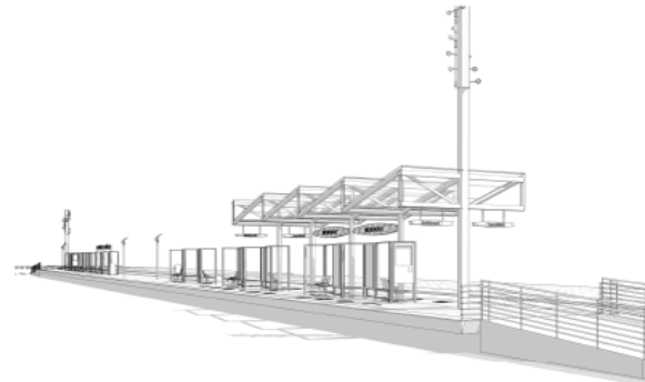
4 PERSPECTIVE VIEW
